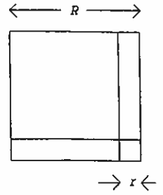
Figure 7. Diagram from which "pro-to-Elements II.7" follows.
