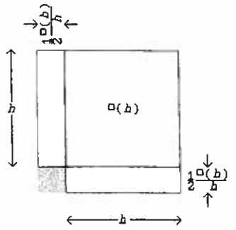
Figure 4. The probable geometrical reasoning behind VAT 6598 #6.
