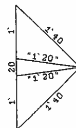
Figure 8. The triangle of YBC 8633.
