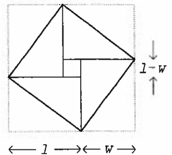
Figure 9, The initial steps of the procedure of Db 2 -146.
