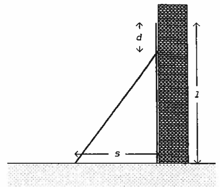
Figure 2. The reed standing and leaned against the wall.
