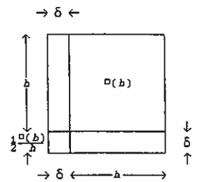
Figure 5. A possible geometrical procedure behind VAT 6598 #7.
