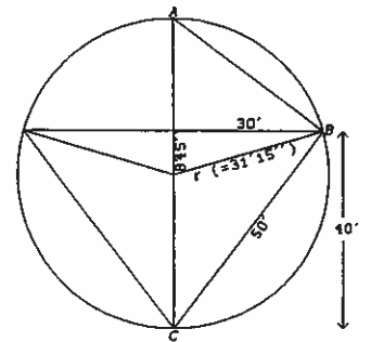
Figure 6. Redrawing of the triangle with circumscribed circle from TMS I
