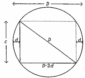
Figure 3. The circle of BM 85194 rev. I 33–43, with chord and descent.
